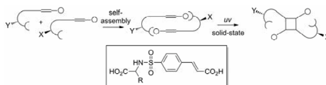
Scheme 1 Design strategy (top) and molecular targets (bottom) for the construction of photoreactive sulfonamidocinnamic acids.
