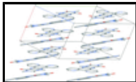
Fig. 2. Packing diagram for the title compound. The molecular planes of alternating stacks of molecules are oriented at 12.46 (2)° relative to one another. The CHCl 3 molecules and H-atoms have been omitted for clarity.
